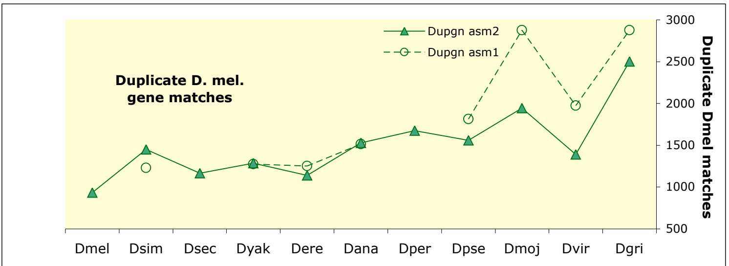
Figure 1 shows number of unique matches from D. melanogaster proteins to Drosophila species genome assemblies. The Dmel column shows the maximum gene count. Figure 2 shows duplicate gene matches. Year 2005 assemblies (asm2) are higher quality, with more unique matches and fewer duplicate matches, than prior assemblies (asm1). Matches are made with tBLASTn of Dmel proteins to the genome assembly DNA. The UCSC Dmel protein reference set (13449 genes with 18941 proteins) differs from the euGenes protein set (single longest protein from each of 13472 genes) so these two are not strictly comparable. UCSC and euGenes are not using same 2004 assemblies.
