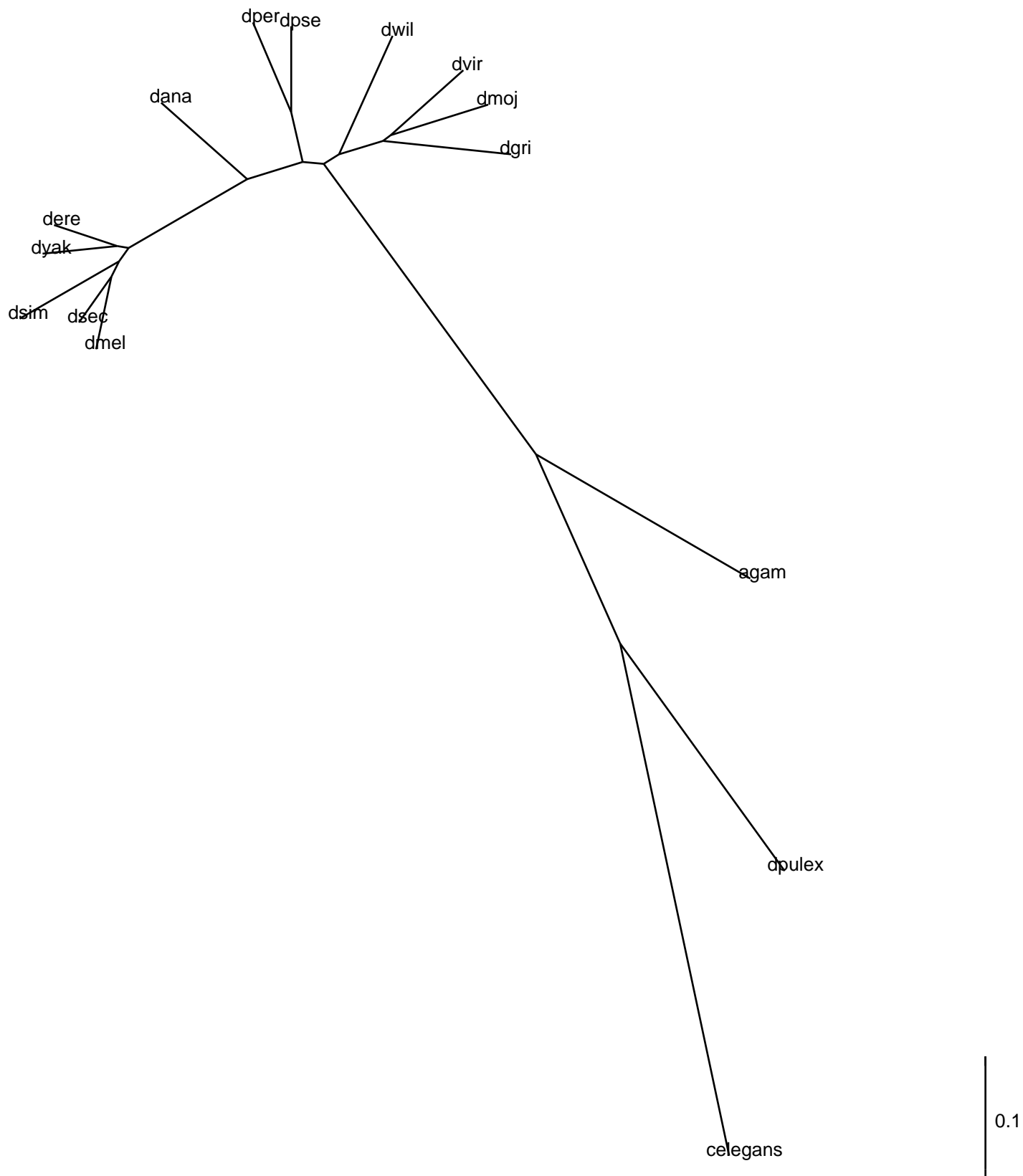
D_melanogaster-gene similarity tree; v5; Fitch/global
